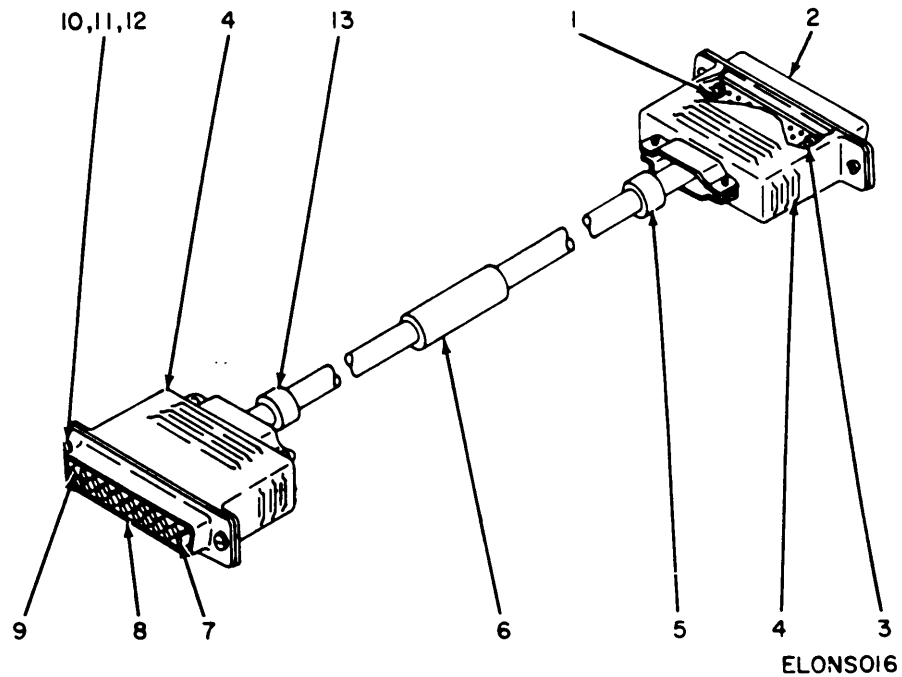
Figure 15. Cable Assembly, Special Purpose, Electrical CX-11735/APM-239A.
