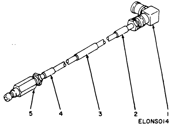
Figure 13. Cable Assembly, Radio Frequency CG-3470/APM-239A.
