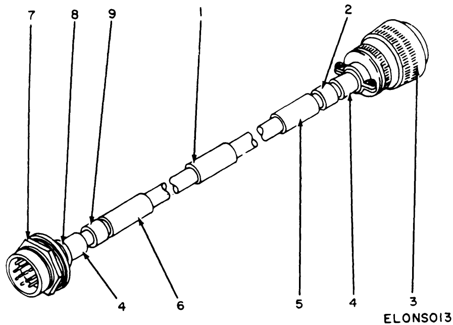
Figure 12. Cable Assembly, Special Purpose, Electrical CX-10910/APM-239A.
