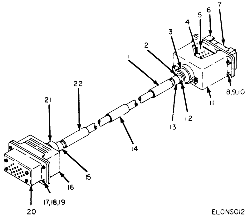
Figure 11. Cable Assembly, Special Purpose, Electrical CX-10907/APM-239A.
