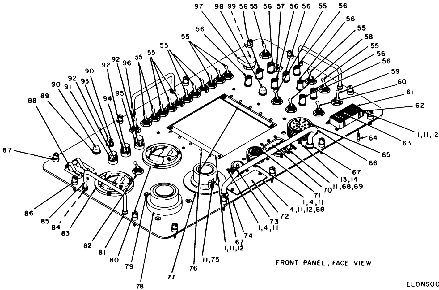
Figure 4. Panel Assembly, Test Set 119067-1 (Sheet 2 of 2).
