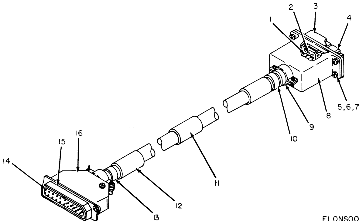
Figure 7. Cable Assembly, Special Purpose, Electrical CX-10905/APM-239A.
