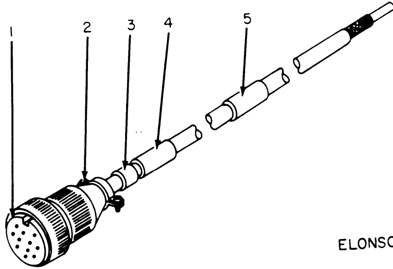
Figure 8. Cable Assembly, Power, Electrical CX-10926/APM-239A.
