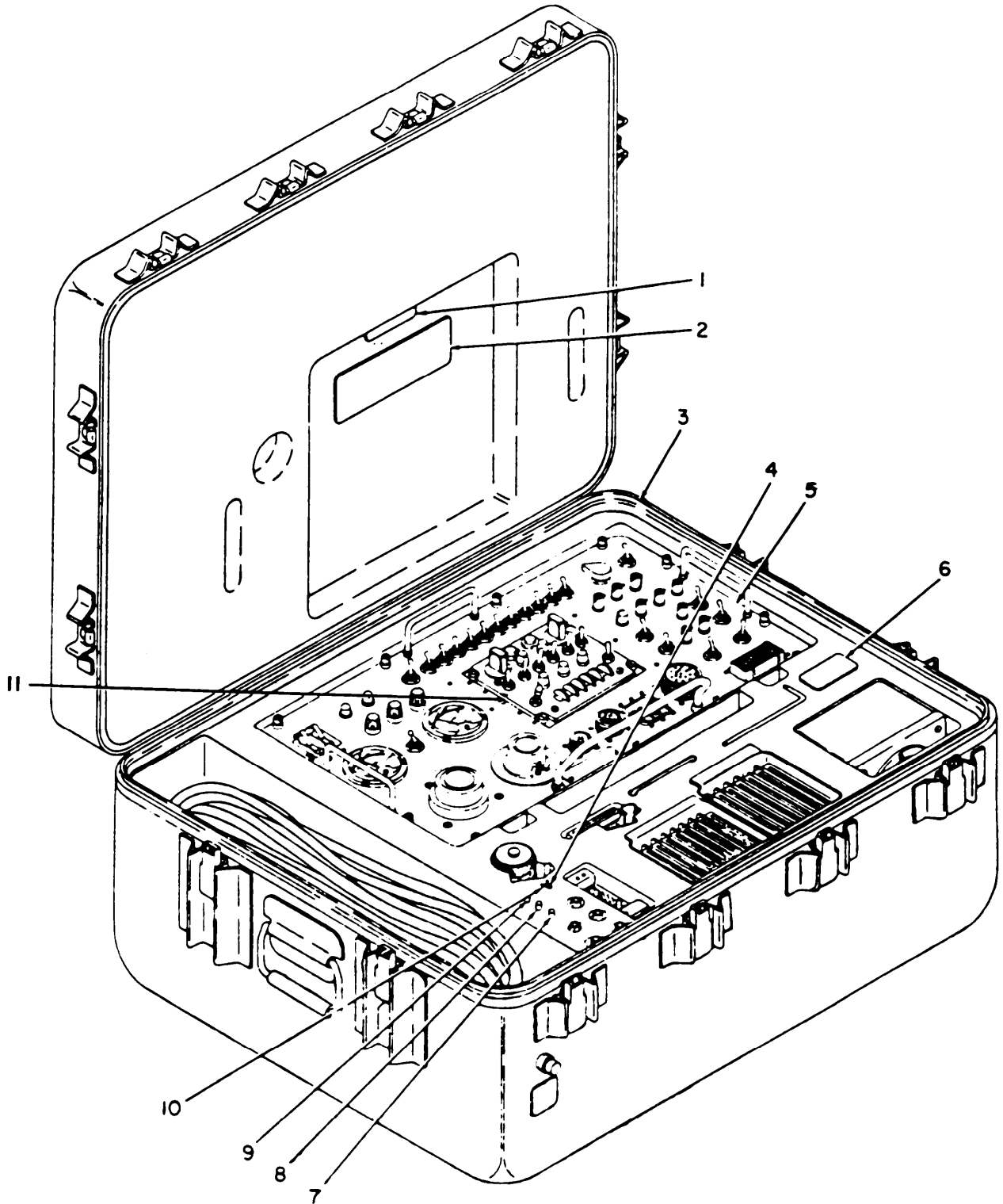
Figure 2. Test Set, Transponder Set, AN/APM-239A, Interior View.
