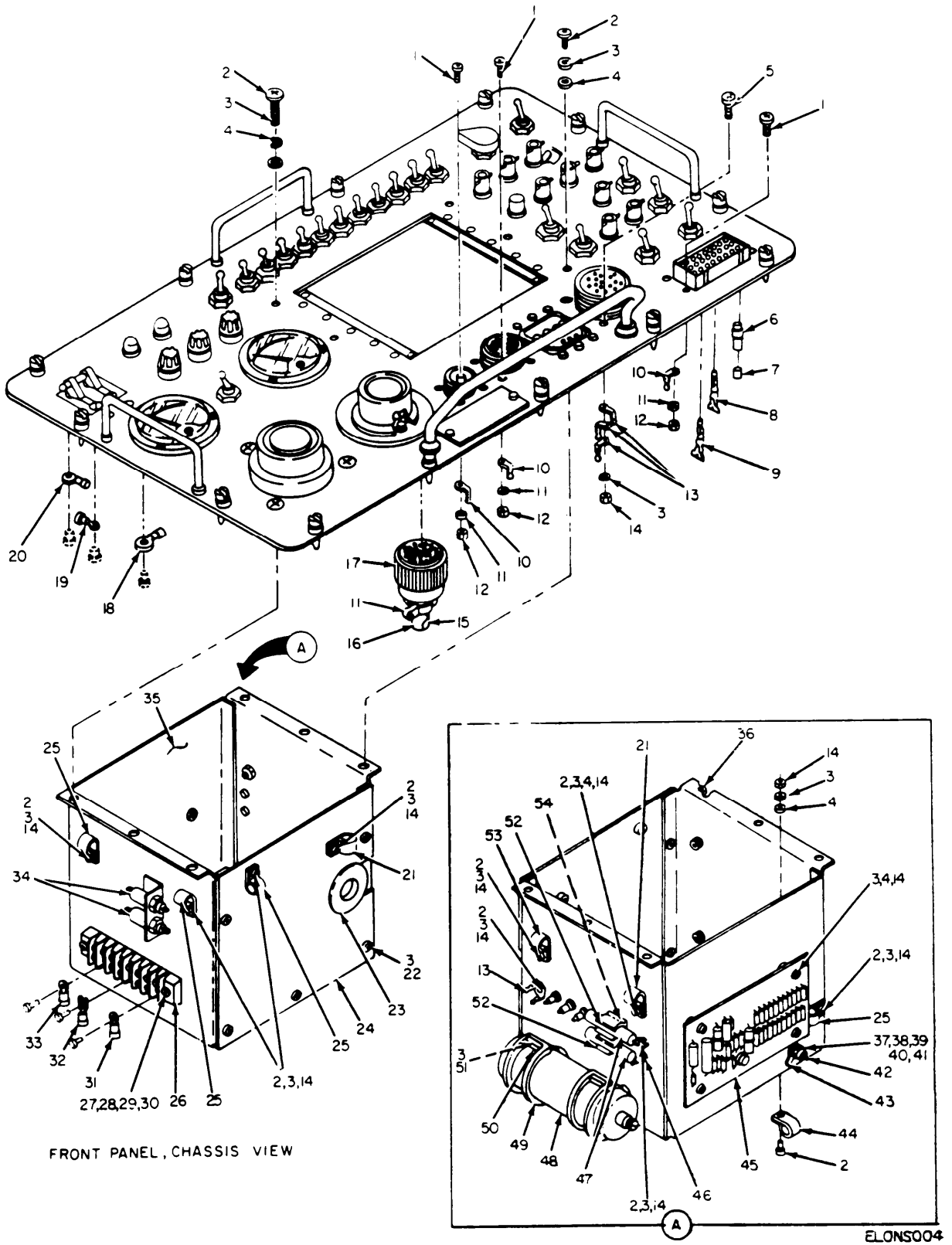
Figure 4. Panel Assembly, Test Set 119067-1 (Sheet 1 of 2).
