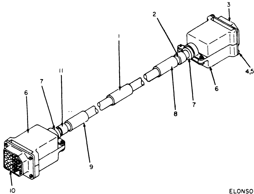
Figure 9. Cable Assembly, Special Purpose, Electrical CX-10908/APM-239A.
