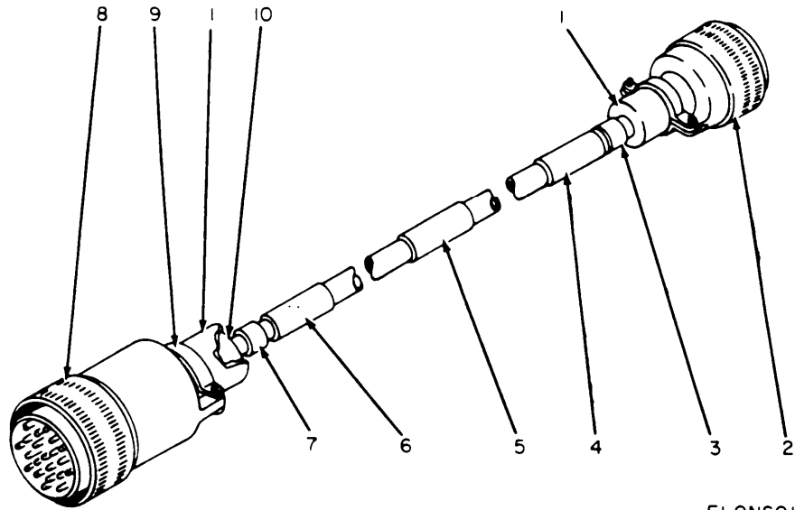
Figure 10. Cable Assembly, Special Purpose, Electrical CX-10909/APM-239A.
