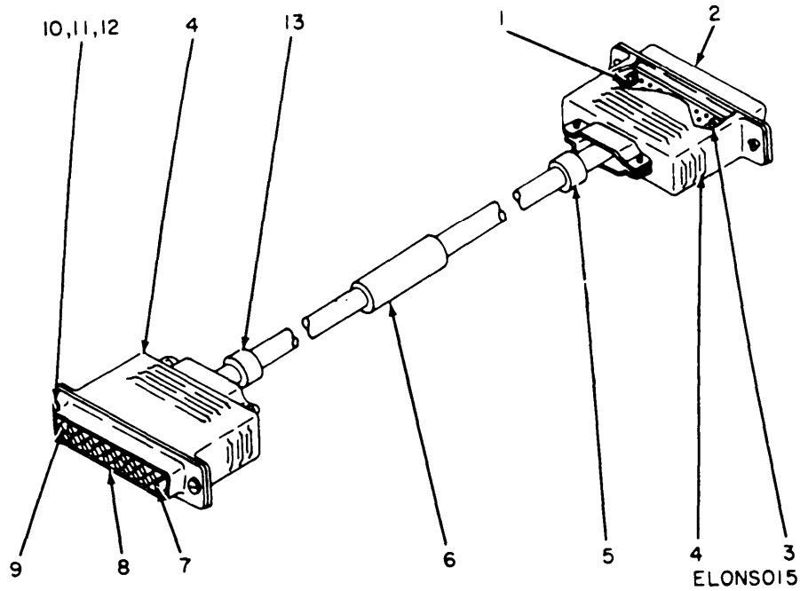
Figure 14. Cable Assembly, Special Purpose, Electrical CX-11734/APM-239A.
