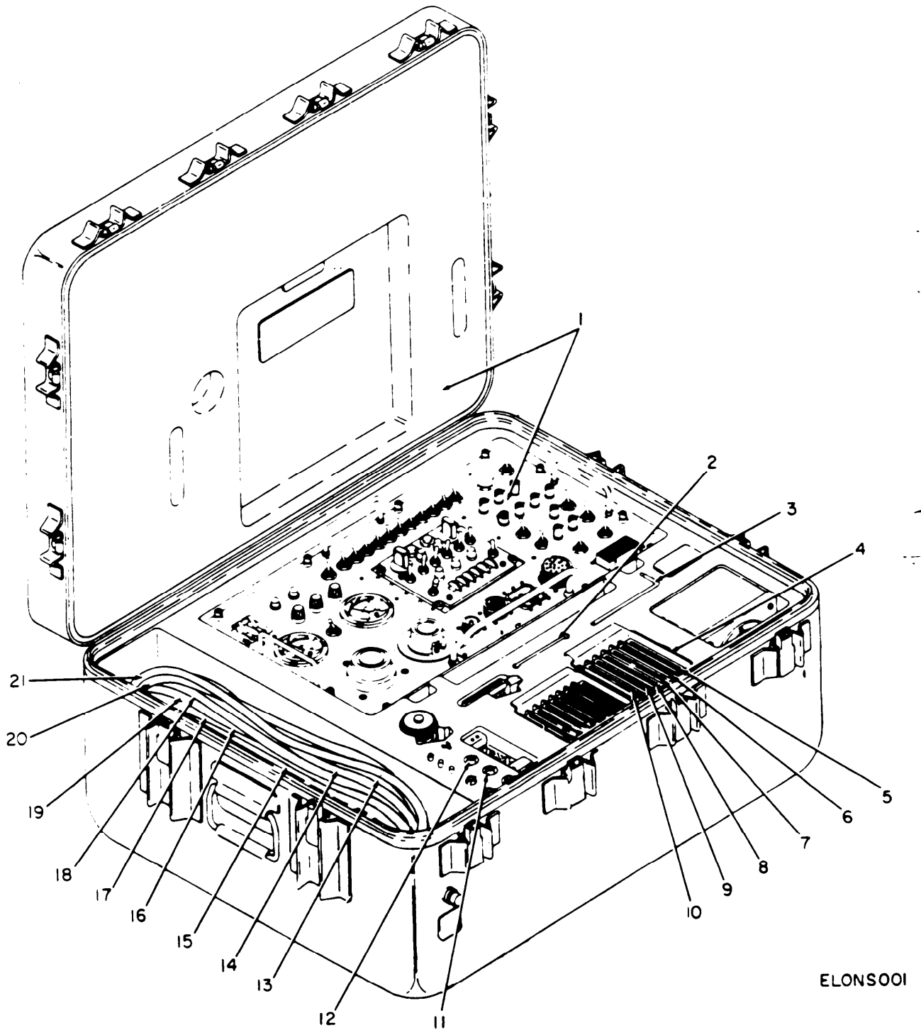
Figure 1. Test Set, Transponder Set AN/APM-239A.
